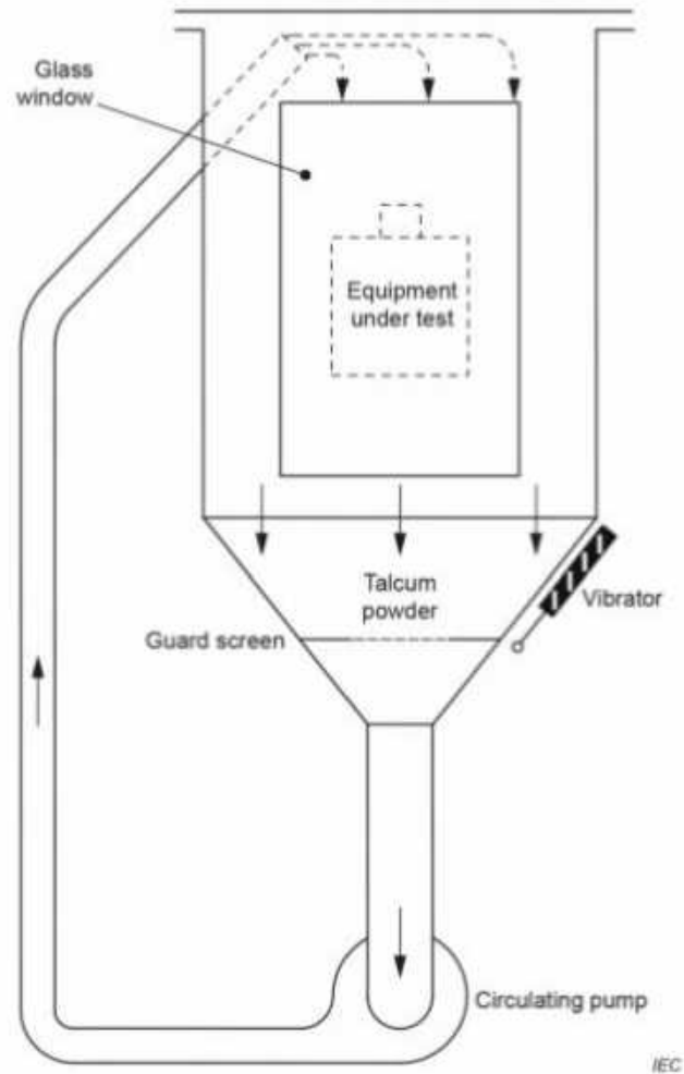
Figure 40 – Apparatus for proving protection against dust
