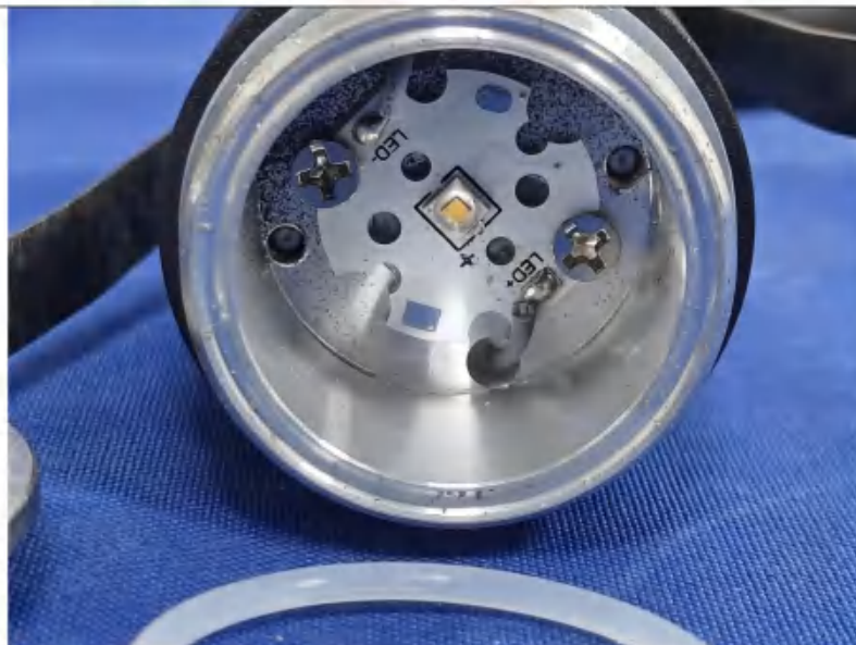
Photo 6: Test result of IP6X and IPX7 test
