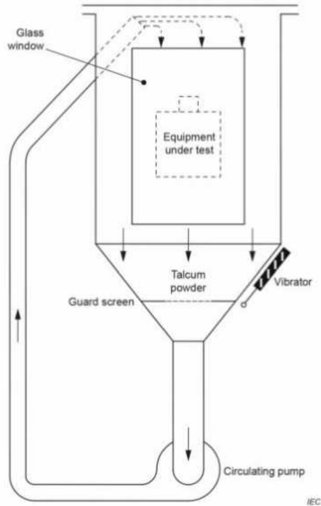
Figure 40 – Apparatus for proving protection against dust
